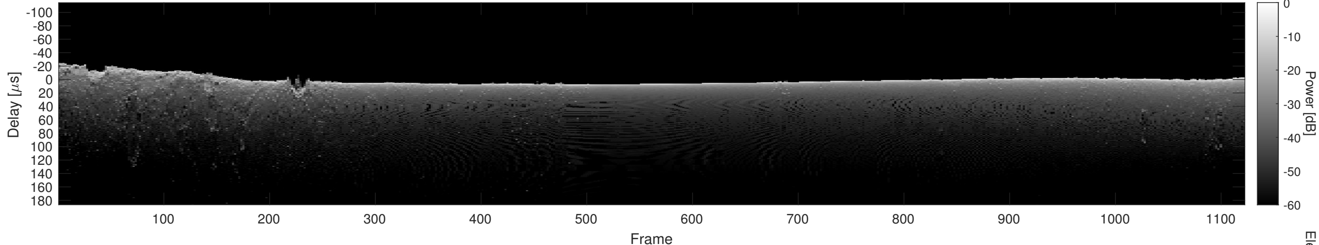
Orbit 18516, Cluttergram
