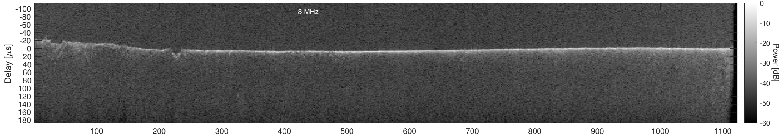
Orbit 18516, Cluttergram
