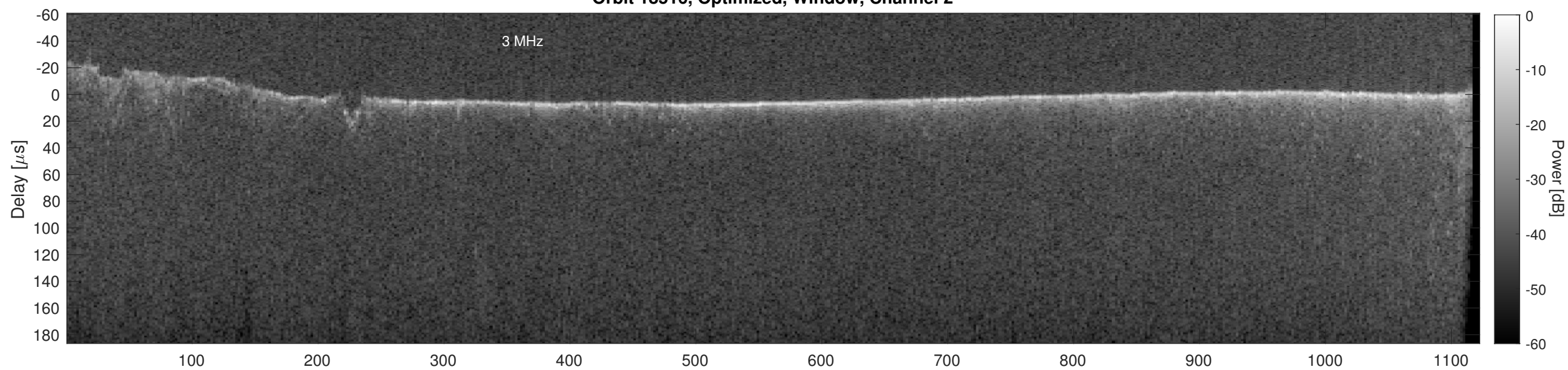
Orbit 18516, Cluttergram
