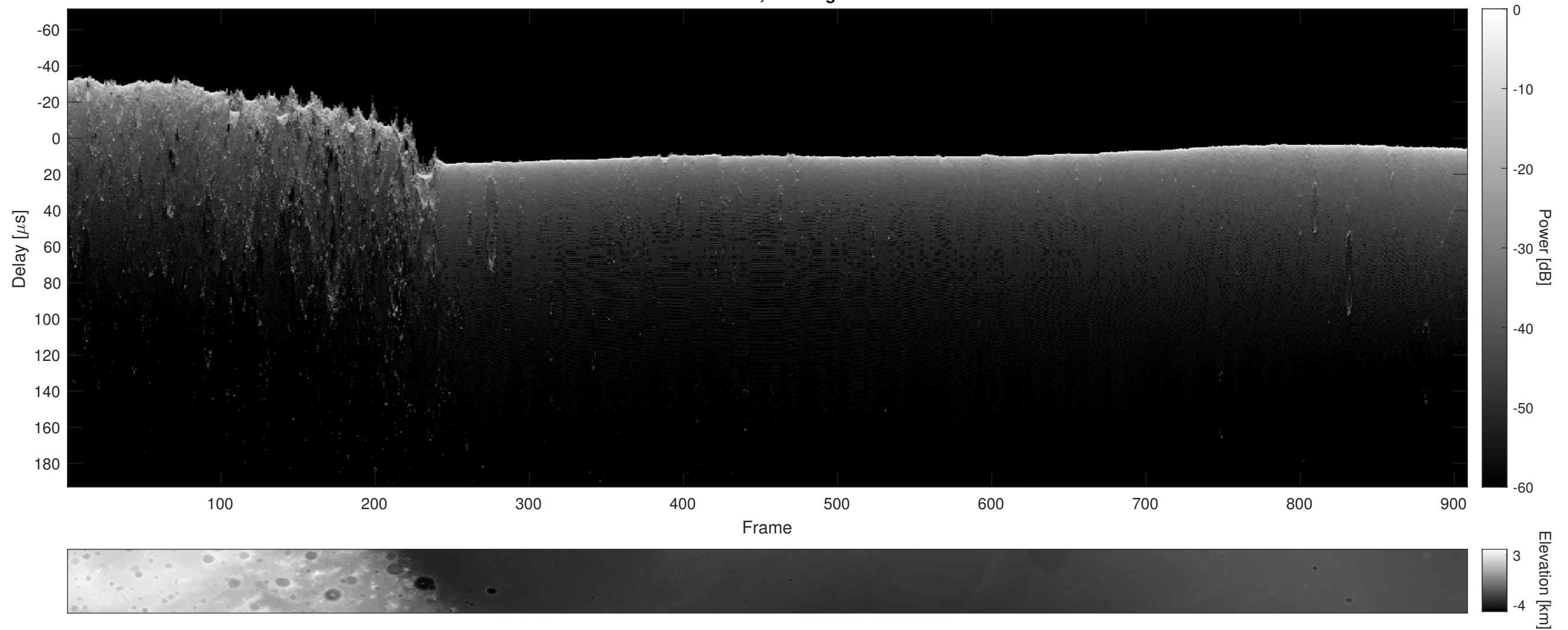
Orbit 18517, Cluttergram
