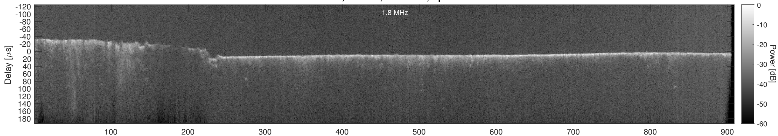
Orbit 18517, Cluttergram
