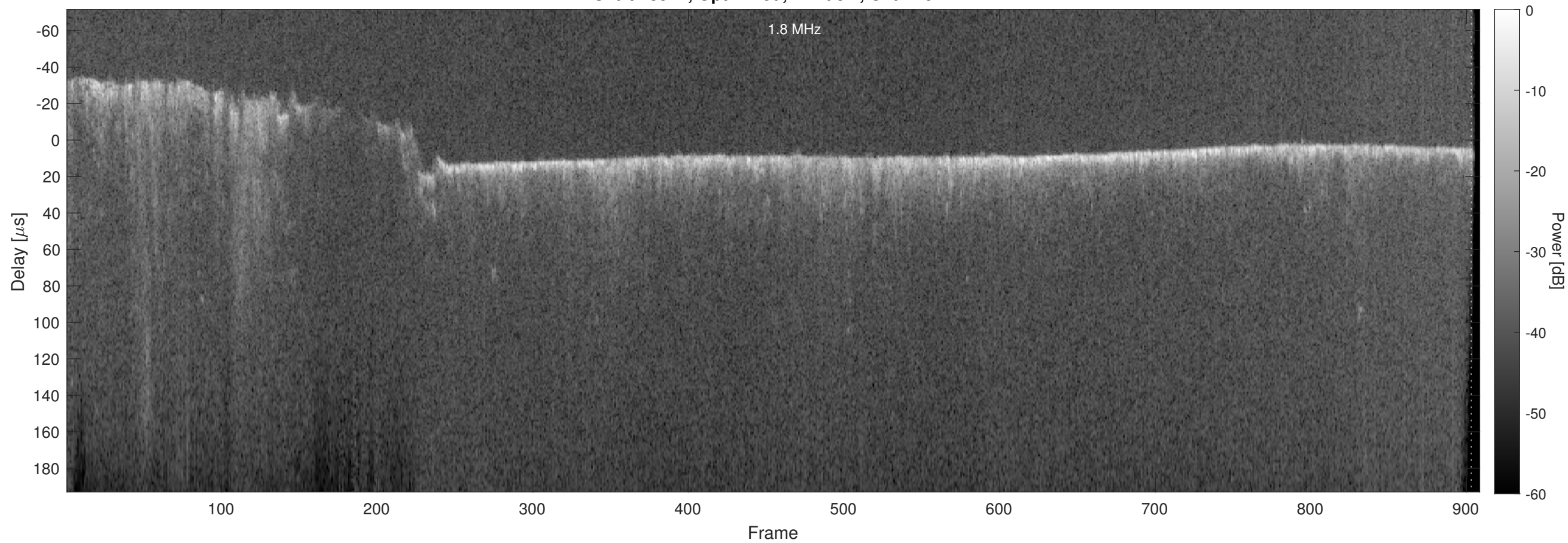
Orbit 18517, Optimized, Window, Channel 2
