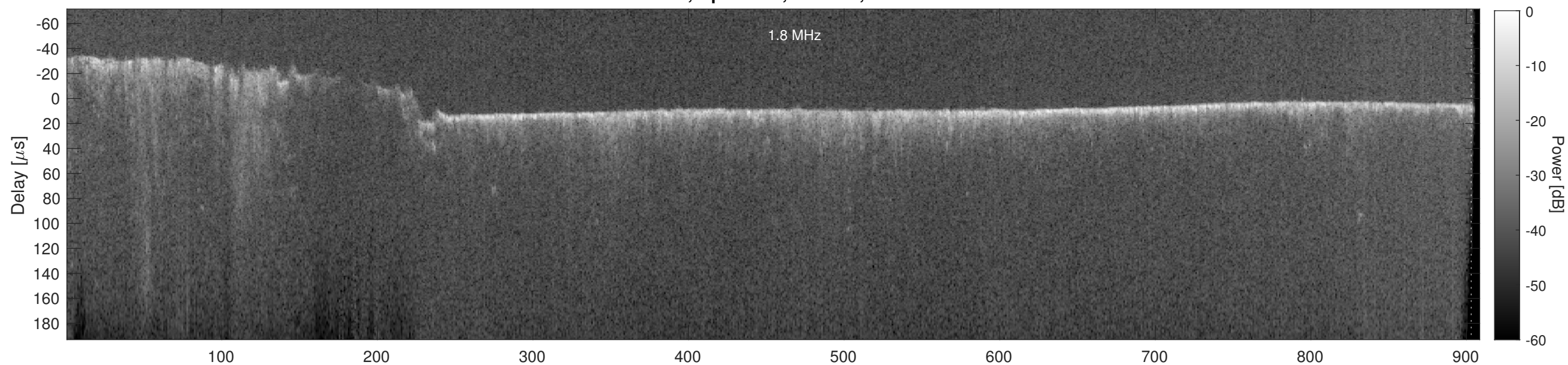
Orbit 18517, Cluttergram
