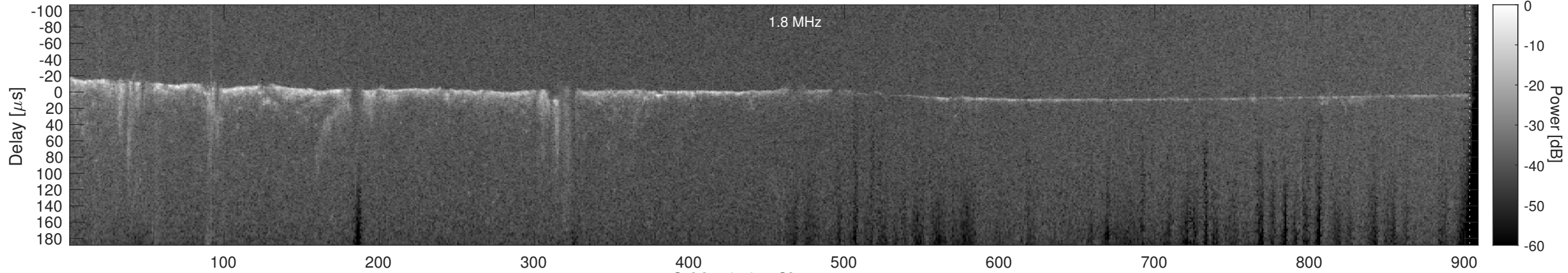
Orbit 18525, Cluttergram
