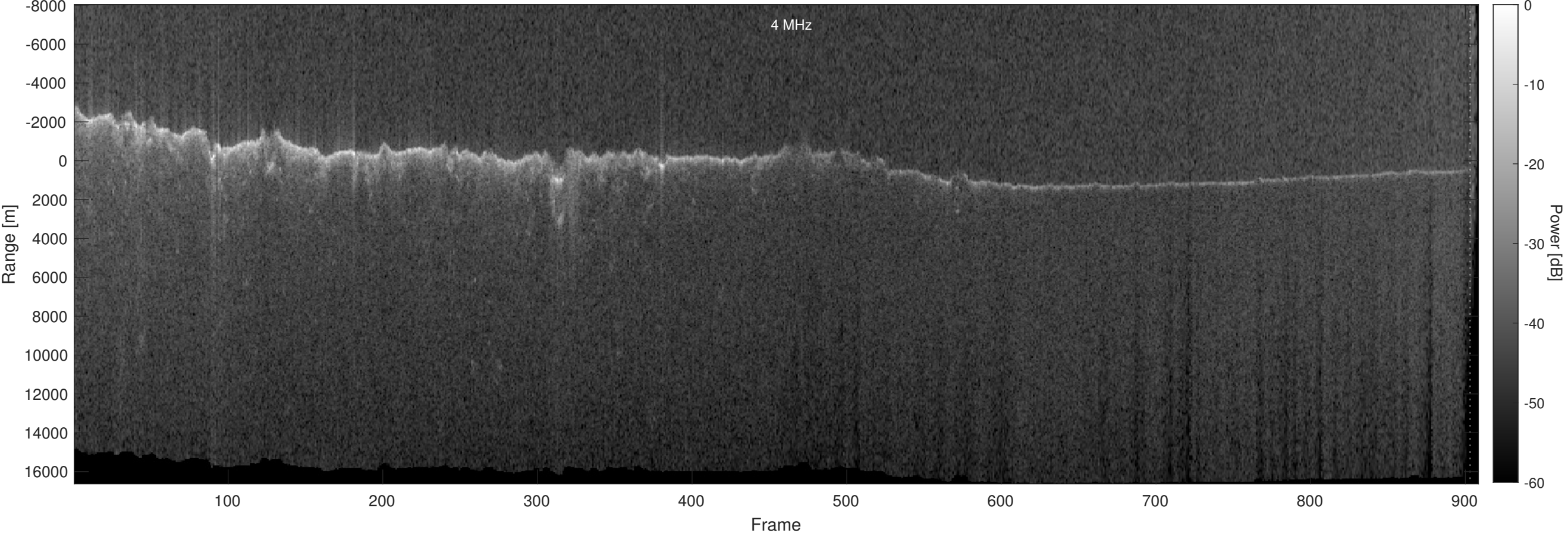
Orbit 18525, Optimized, No Window, Depth-Corrected, Channel 2
