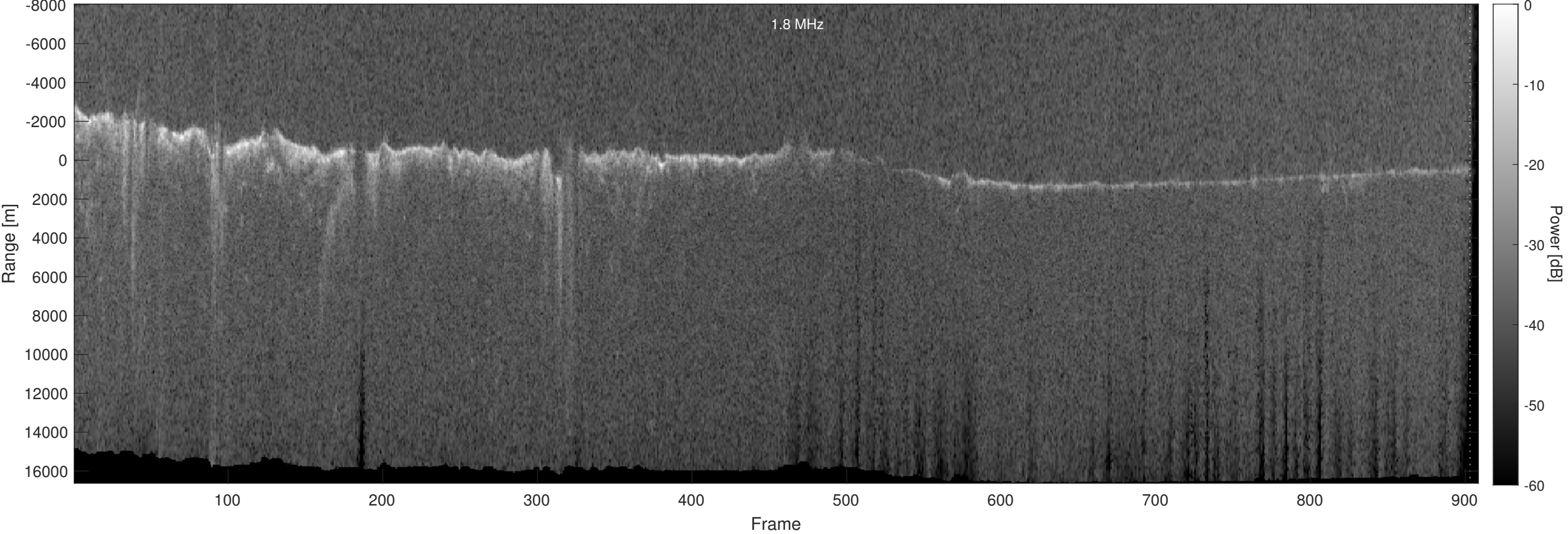
Orbit 18525, Optimized, Window, Depth-Corrected, Channel 2
