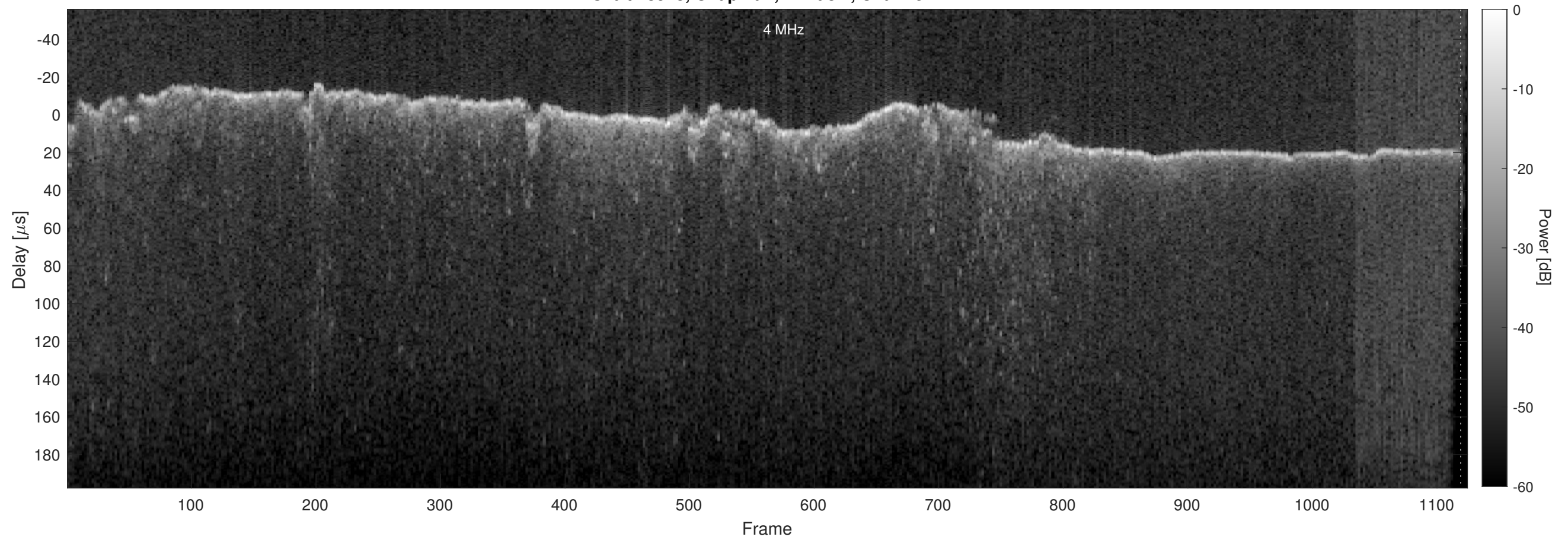
Orbit 18528, Chapman, Window, Channel 2
