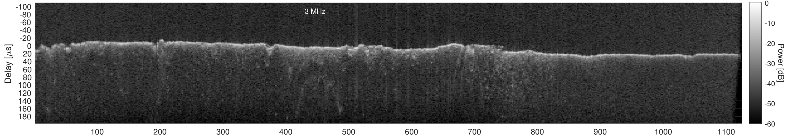
Orbit 18528, Window, Channel 2, Chapman
