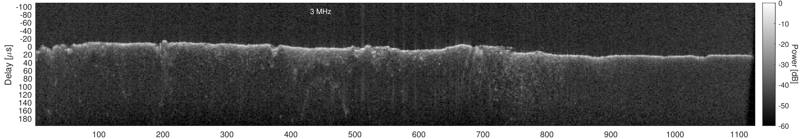
Orbit 18528, Window, Channel 2, Optimized
