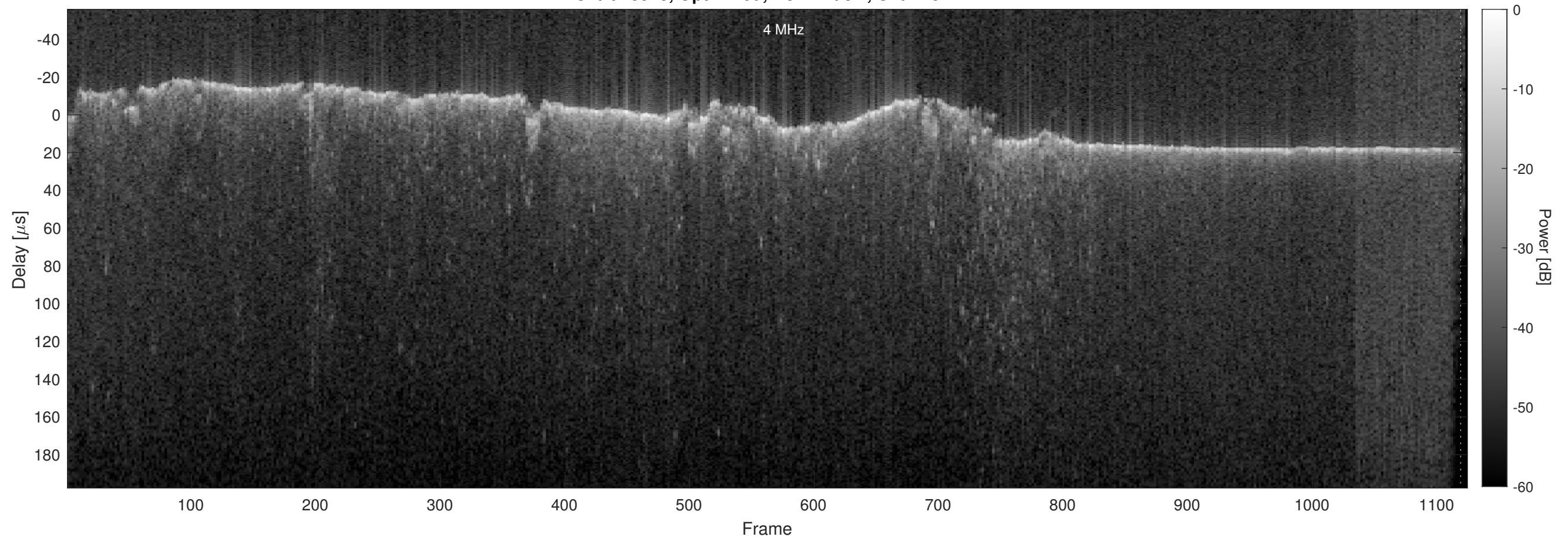
Orbit 18528, Optimized, No Window, Channel 2
