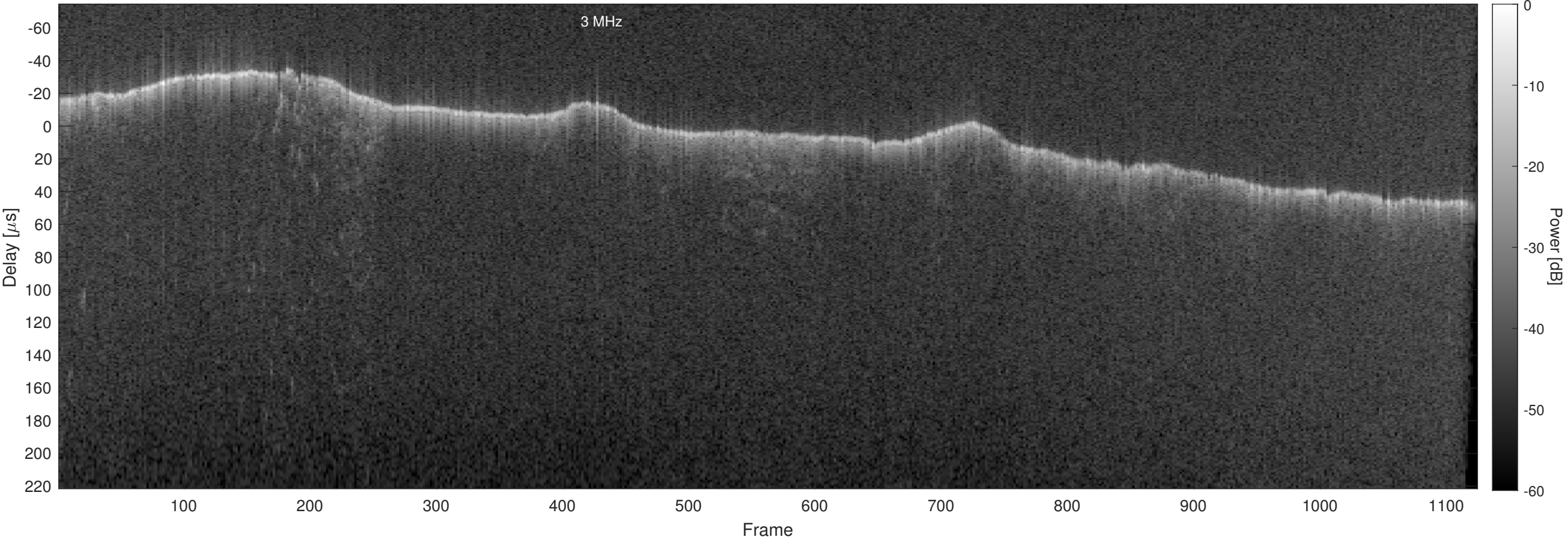
Orbit 18533, Chapman, No Window, Channel 2
