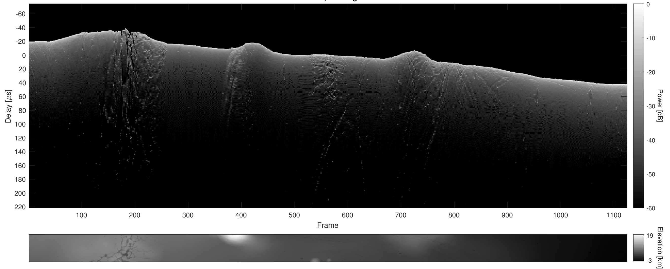
Orbit 18533, Cluttergram
