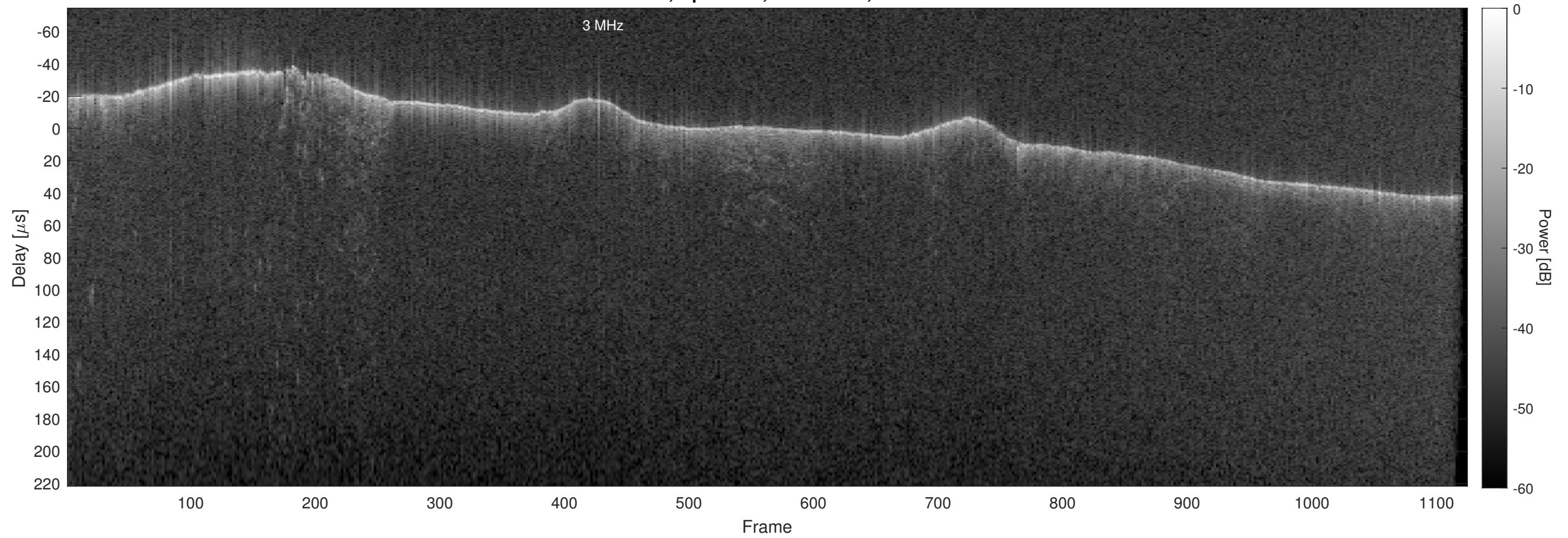
Orbit 18533, Optimized, No Window, Channel 2
