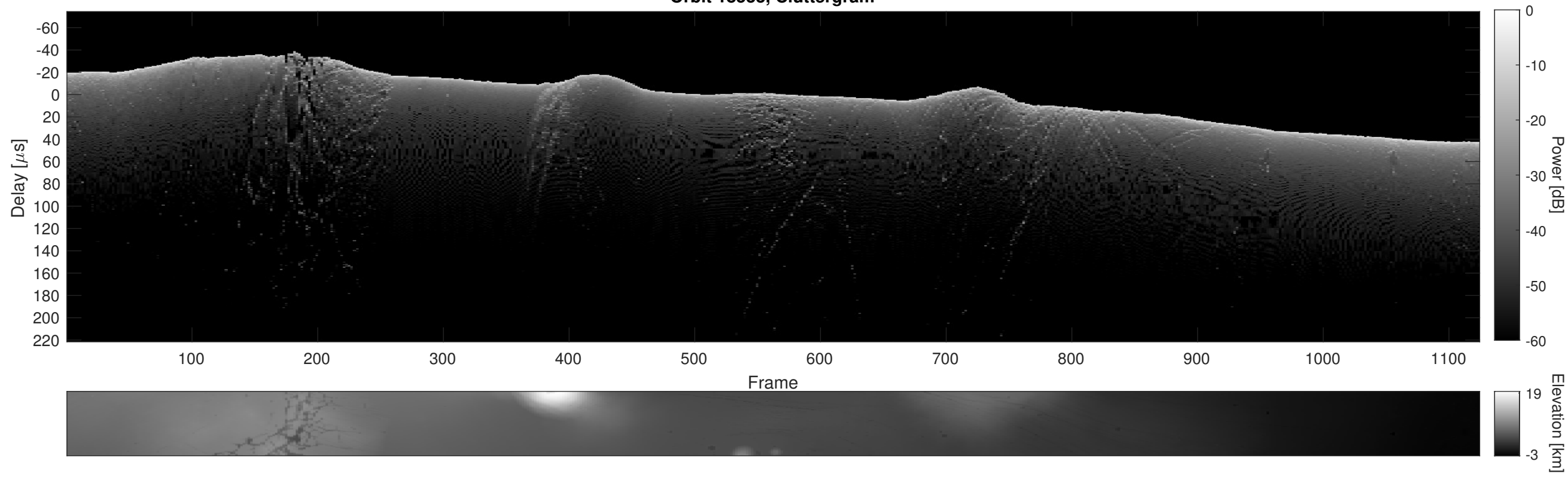
Orbit 18533, Cluttergram
