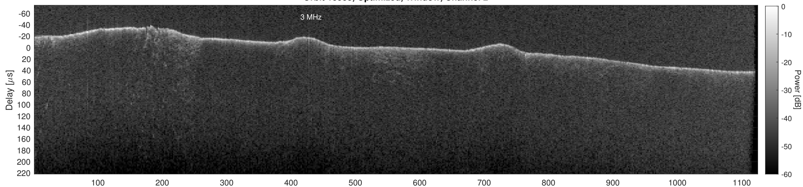
Orbit 18533, Cluttergram
