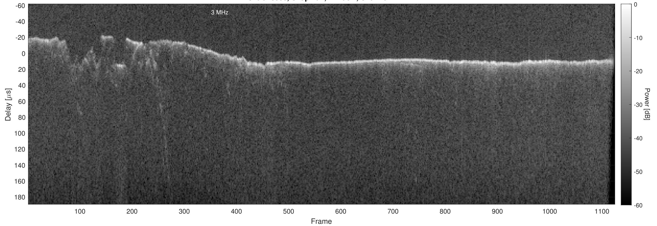
Orbit 18536, Chapman, Window, Channel 2
