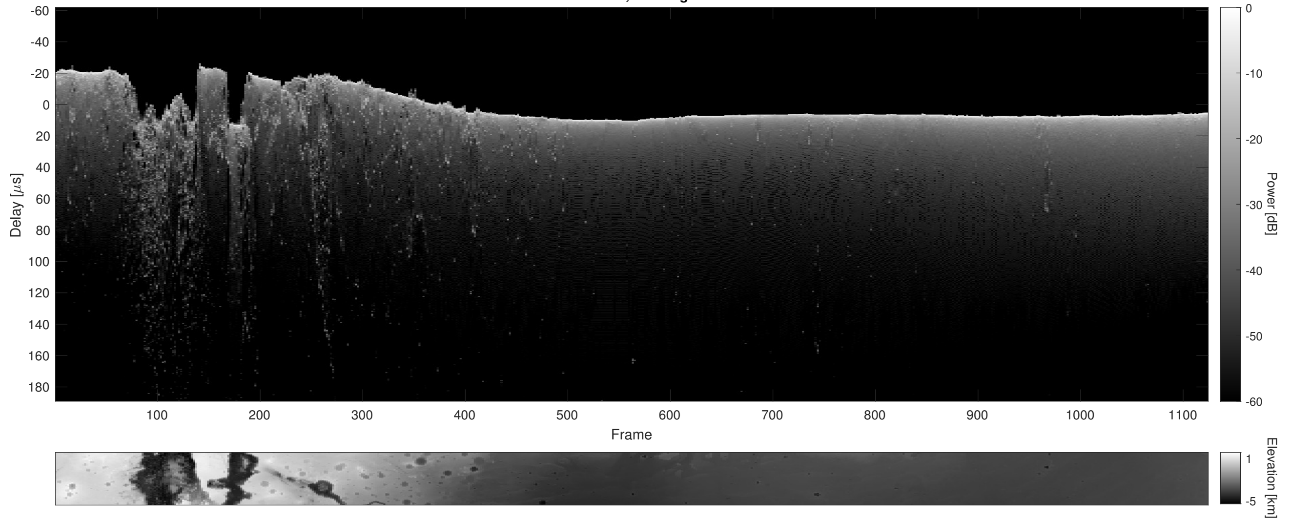
Orbit 18536, Cluttergram
