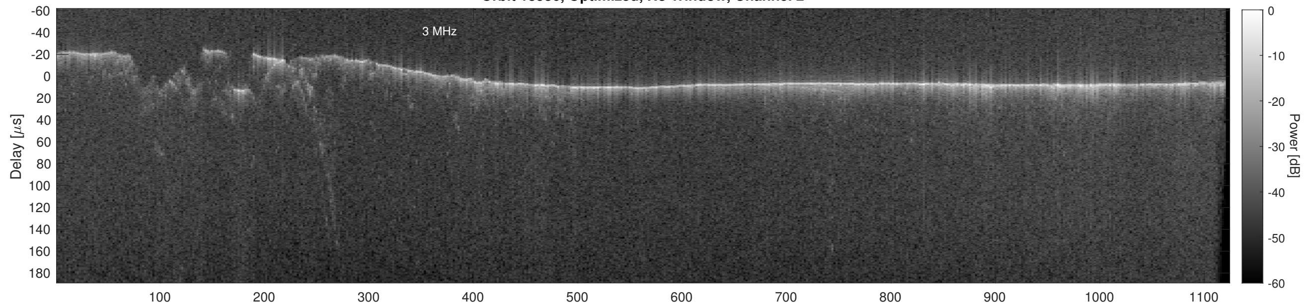
Orbit 18536, Cluttergram
