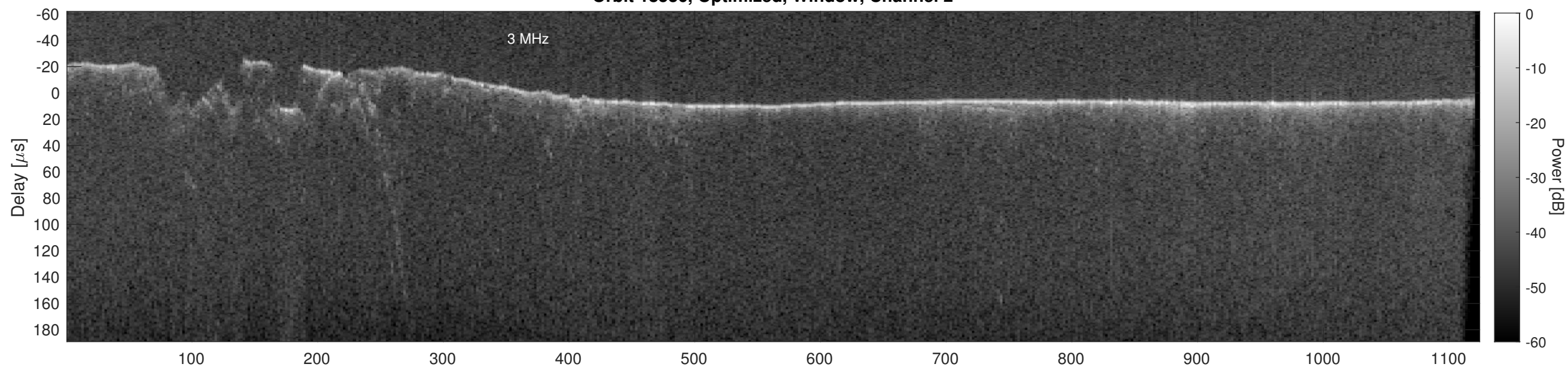
Orbit 18536, Cluttergram
