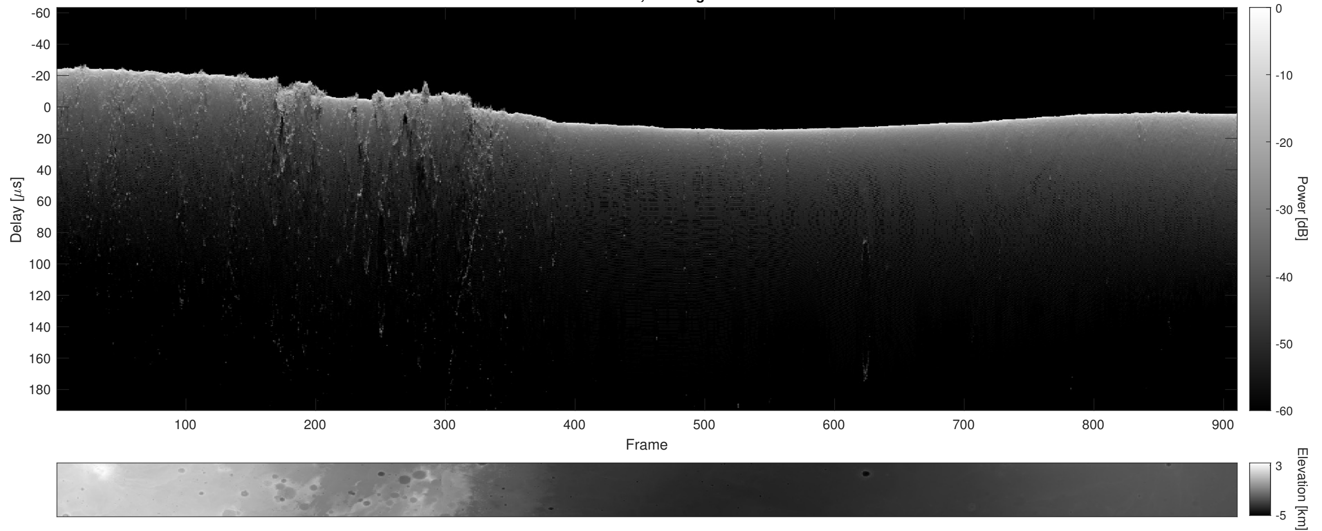
Orbit 18538, Cluttergram
