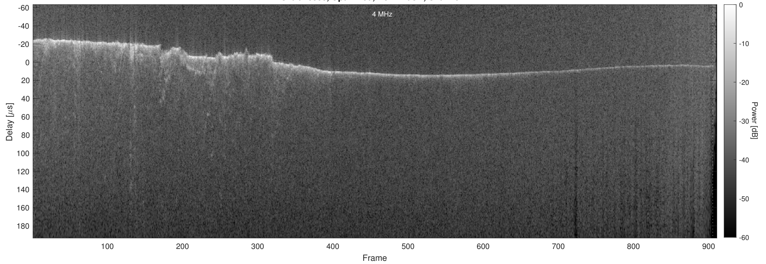
Orbit 18538, Optimized, No Window, Channel 2
