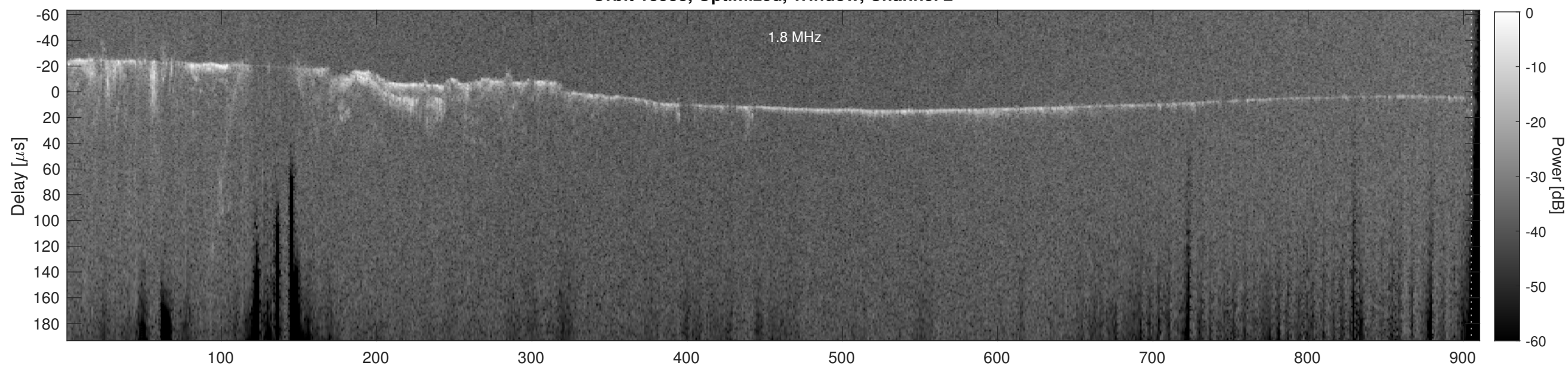
Orbit 18538, Cluttergram
