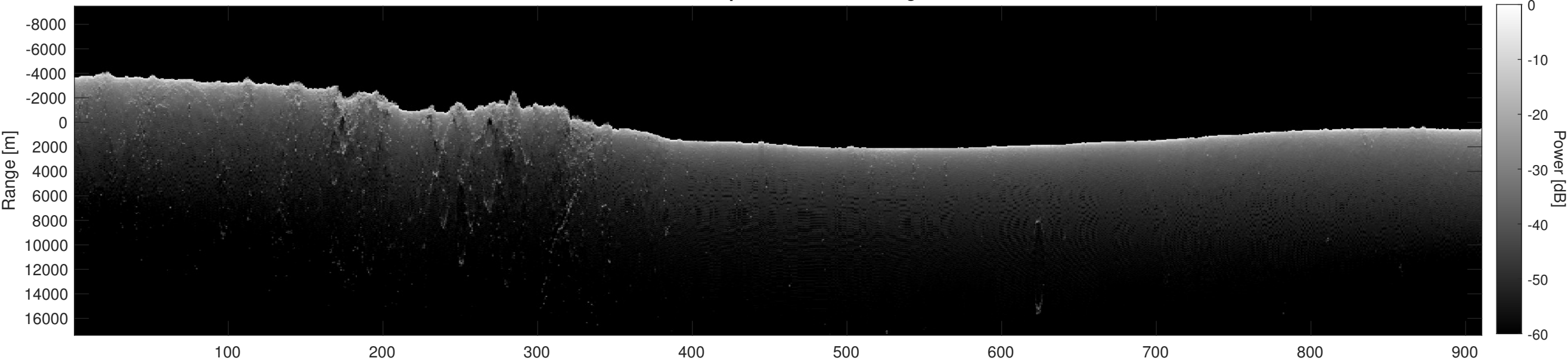
Orbit 18538, Depth-Corrected Cluttergram
