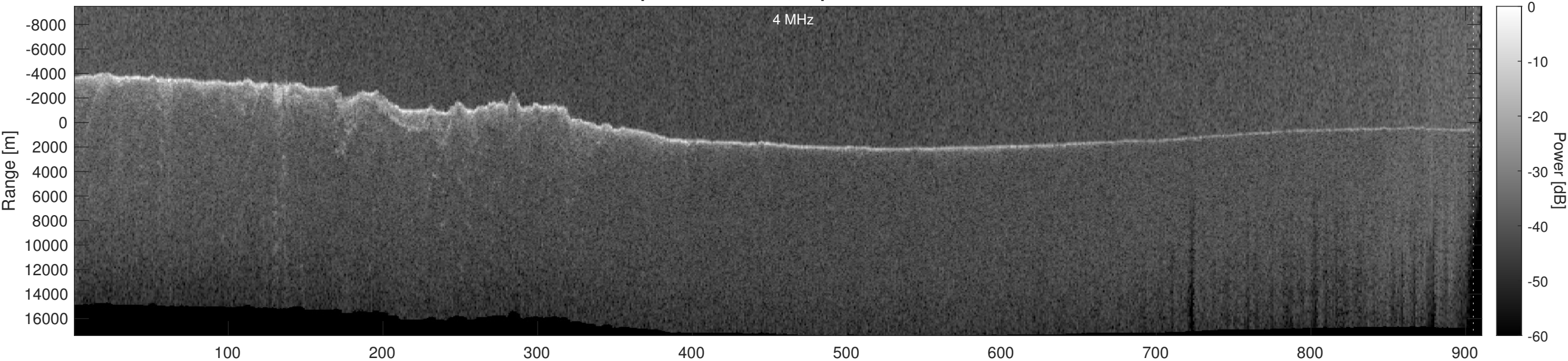
Orbit 18538, Optimized, Window, Depth-Corrected, Channel 2
