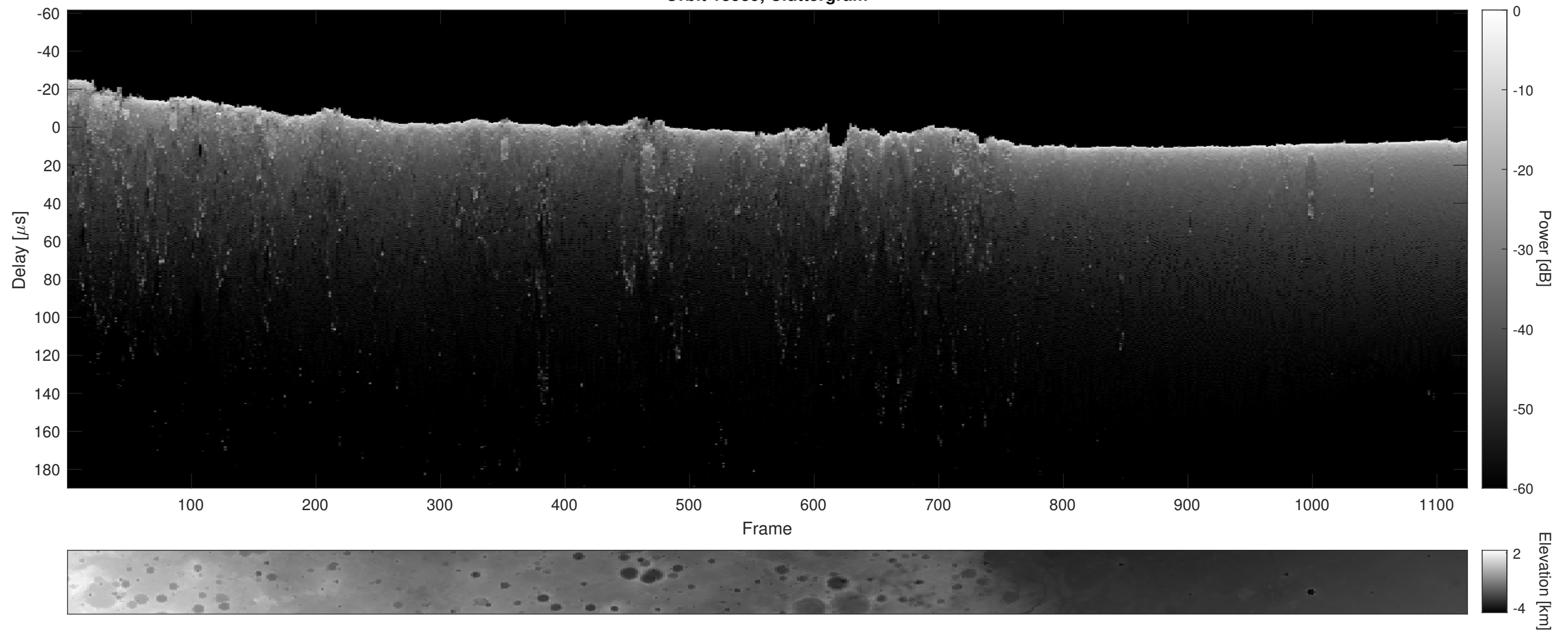
Orbit 18539, Cluttergram
