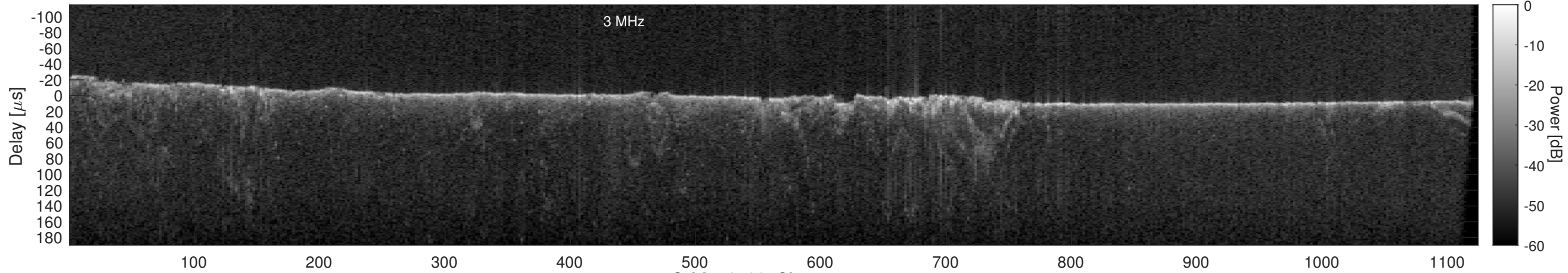
Orbit 18539, Cluttergram
