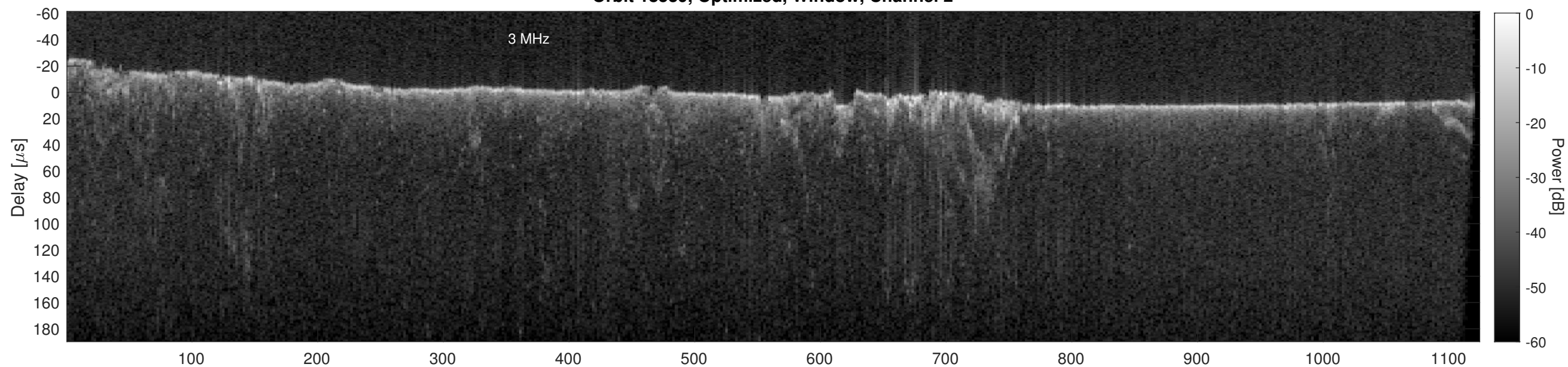
Orbit 18539, Cluttergram
