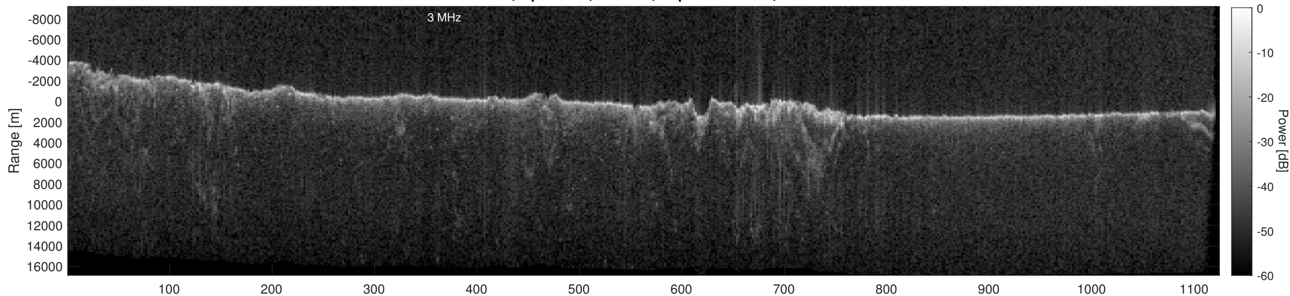
Orbit 18539, Depth-Corrected Cluttergram
