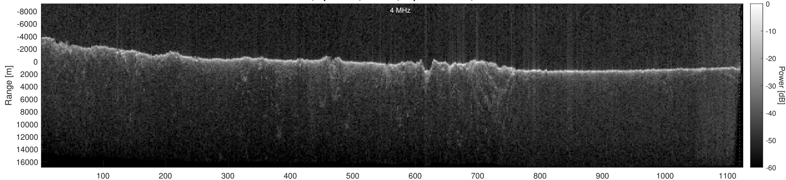
Orbit 18539, Optimized, Window, Depth-Corrected, Channel 2
