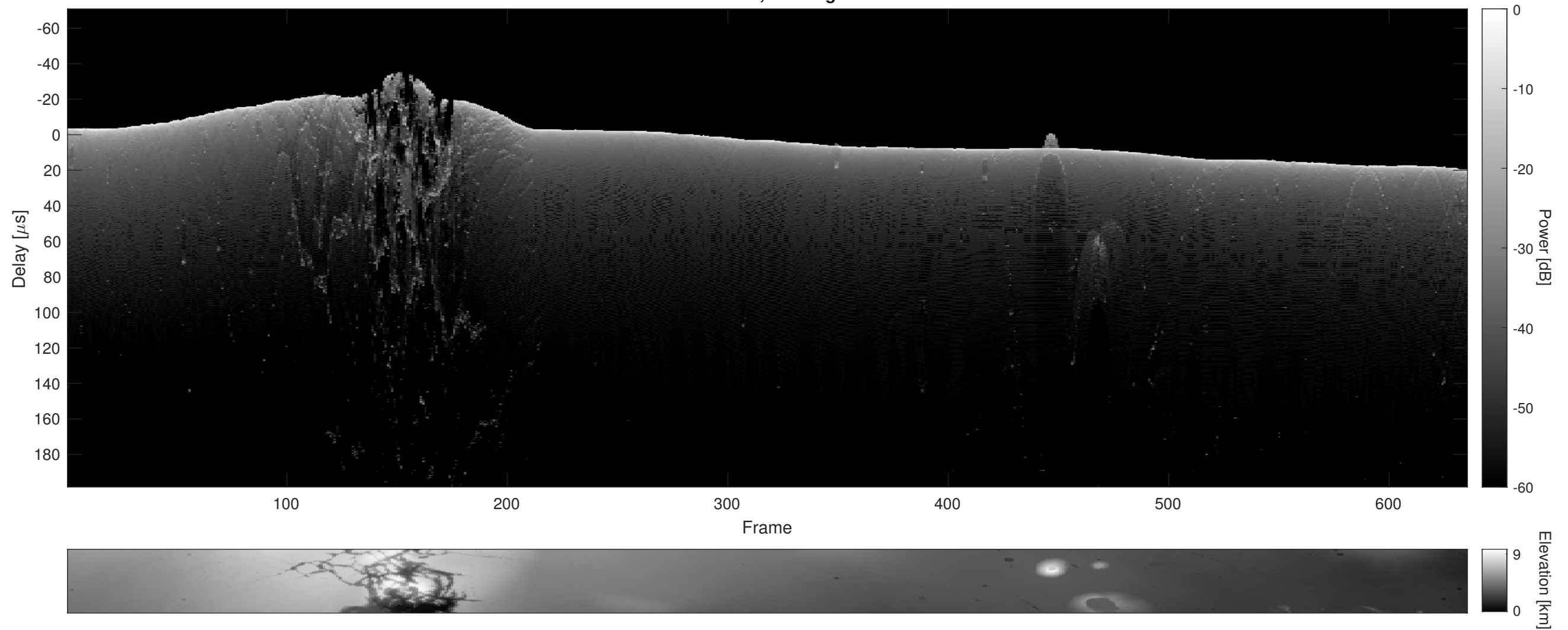
Orbit 18540, Cluttergram
