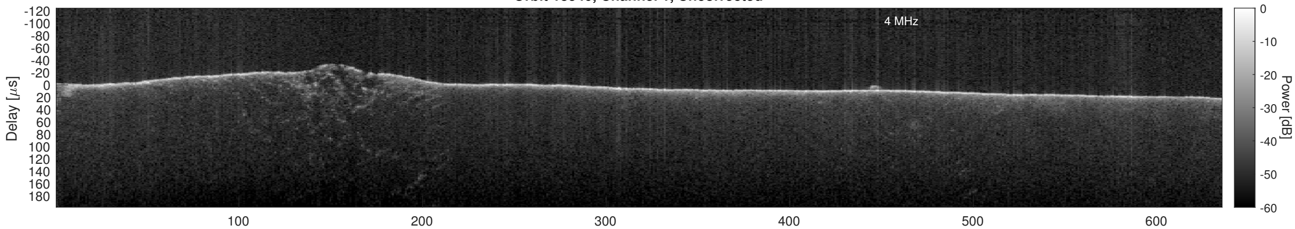
Orbit 18540, Window, Channel 1, Chapman
