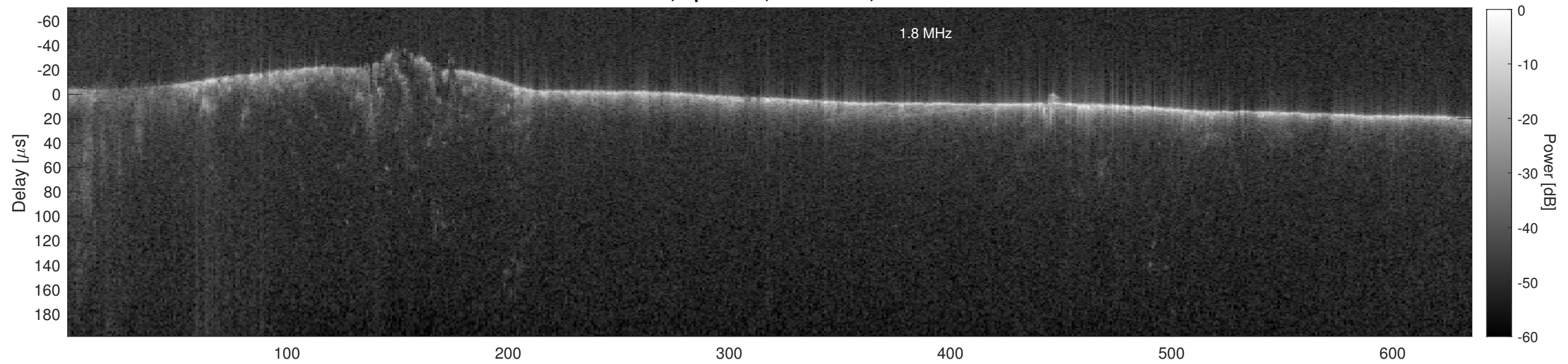
Orbit 18540, Cluttergram
