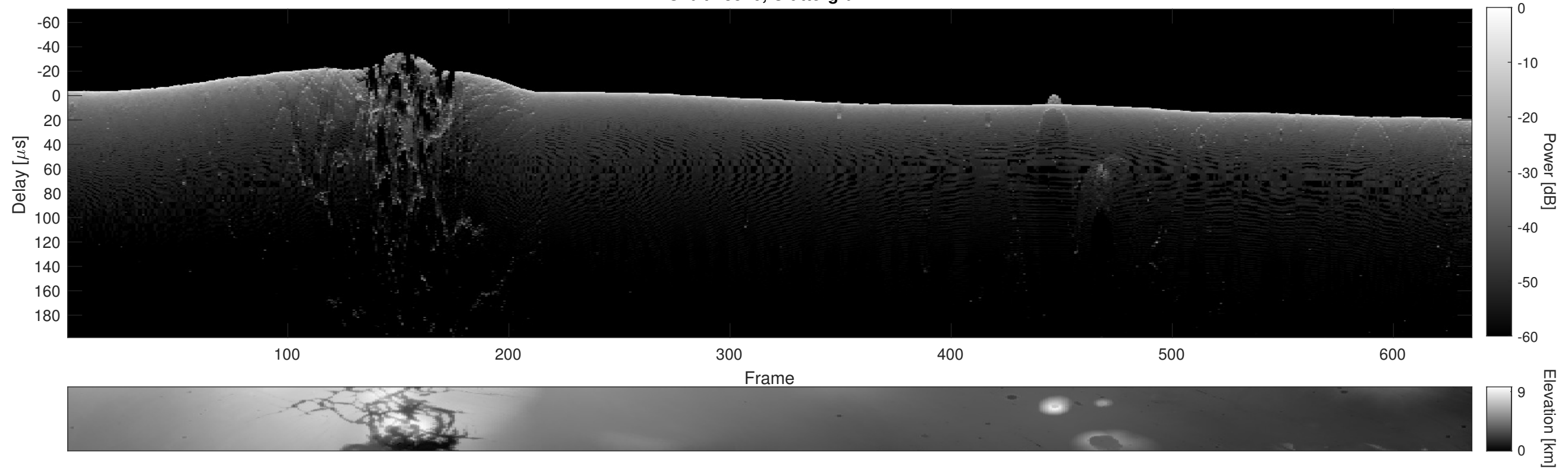
Orbit 18540, Cluttergram
