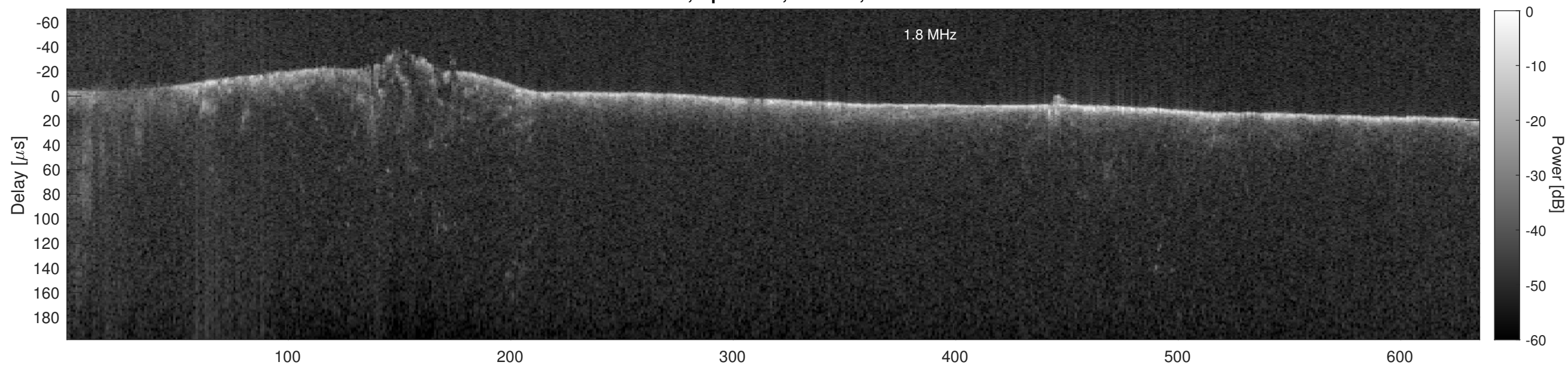
Orbit 18540, Cluttergram
