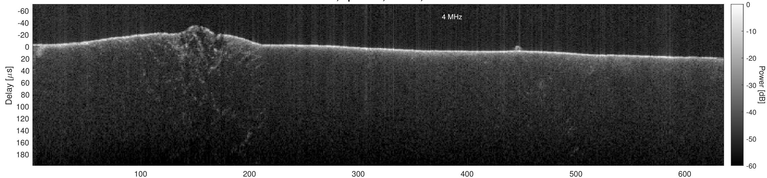
Orbit 18540, Optimized, Window, Channel 2
