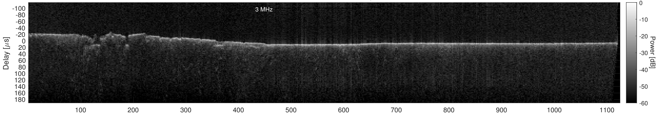
Orbit 18543, Cluttergram
