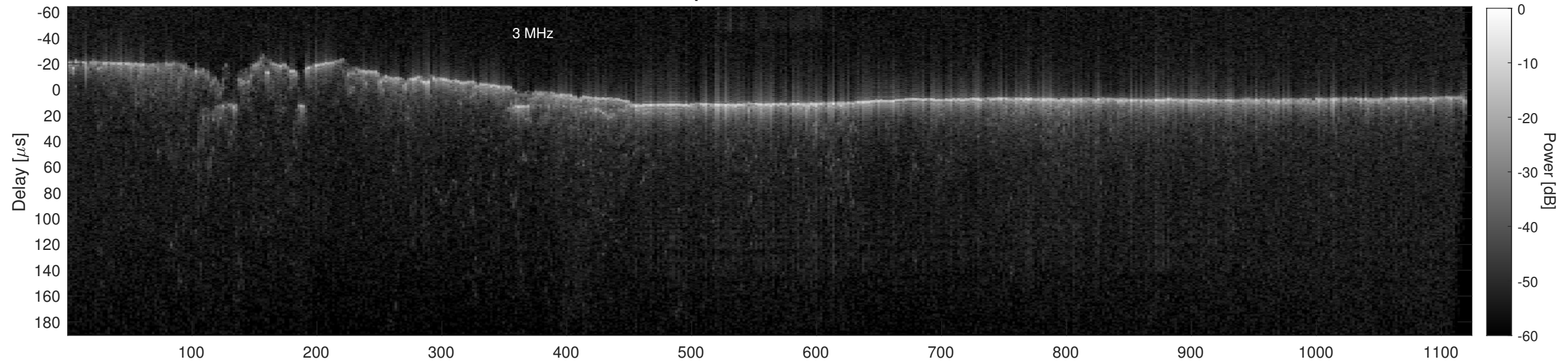
Orbit 18543, Cluttergram
