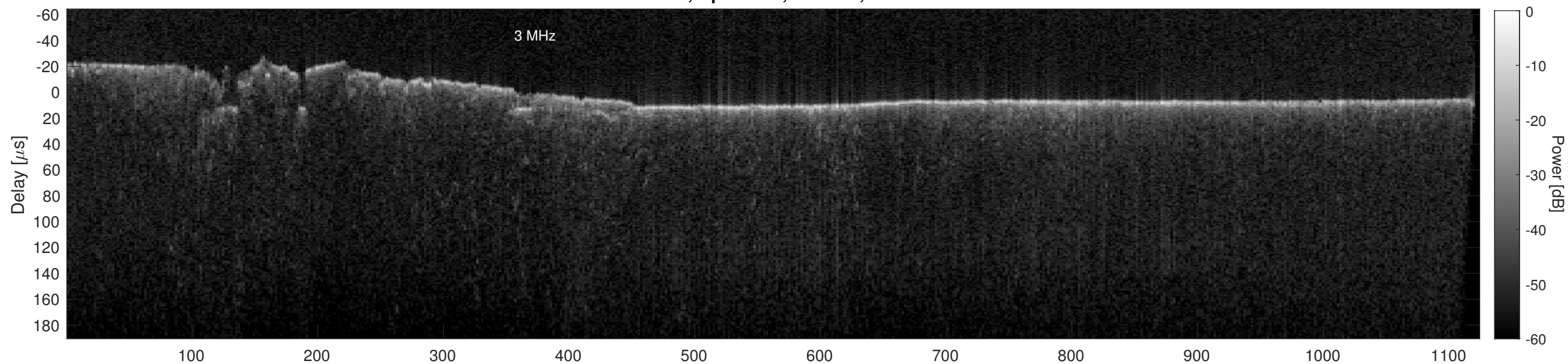
Orbit 18543, Cluttergram
