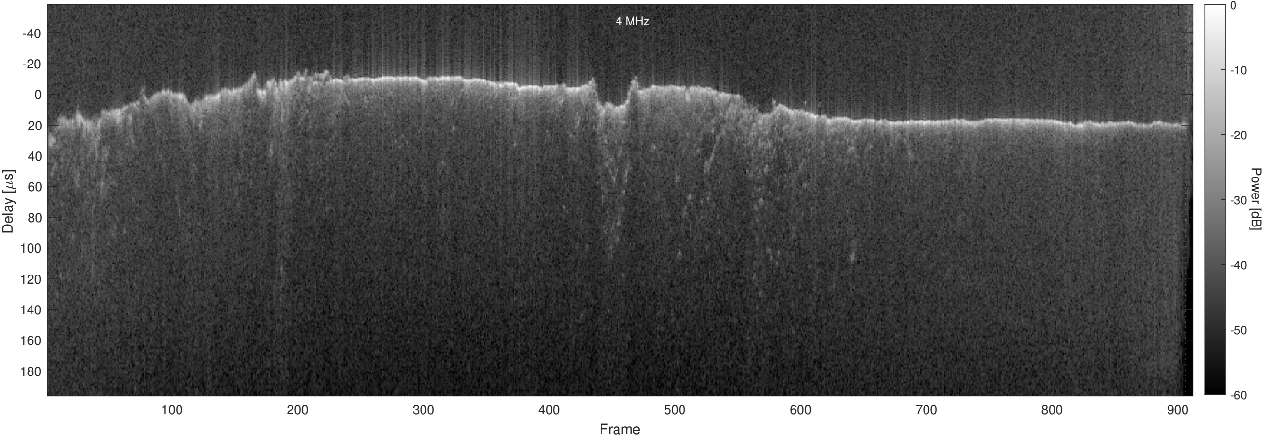
Orbit 18549, Chapman, No Window, Channel 2
