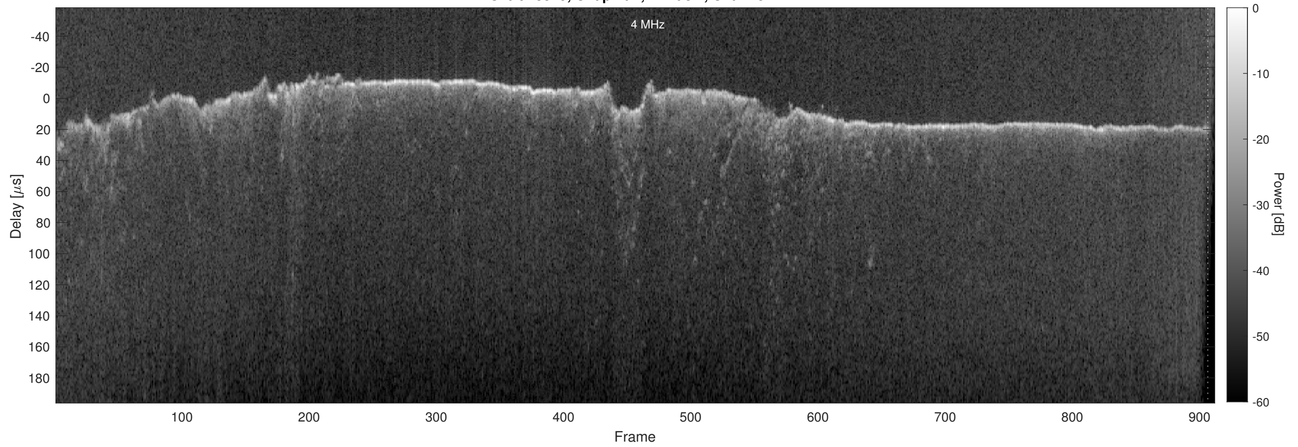
Orbit 18549, Chapman, Window, Channel 2
