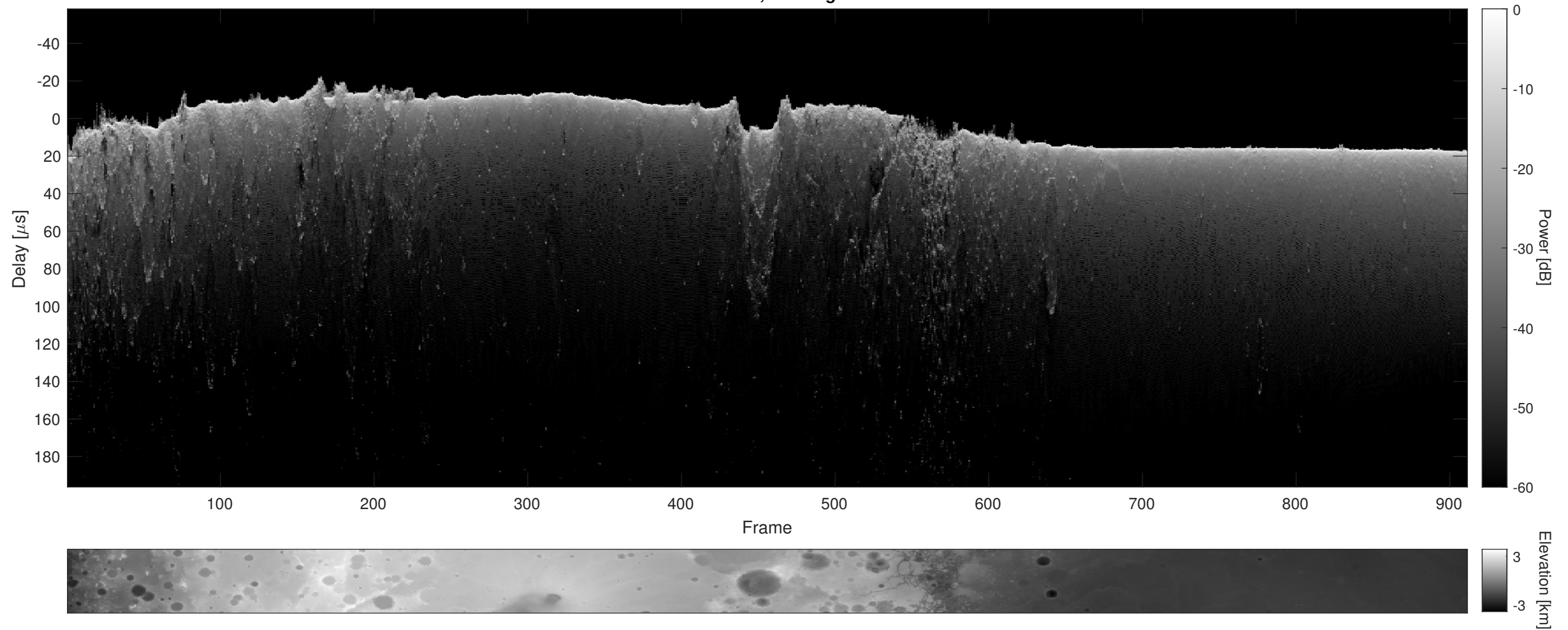
Orbit 18549, Cluttergram
