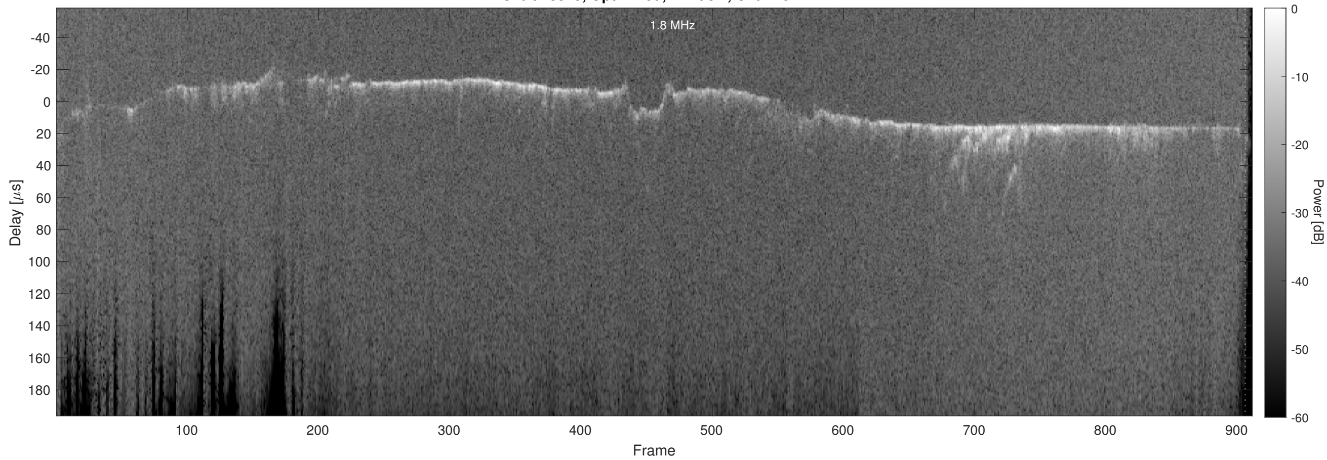
Orbit 18549, Optimized, Window, Channel 2
