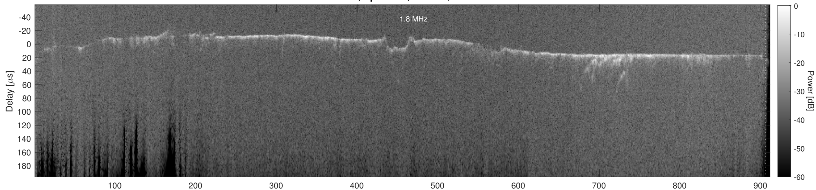
Orbit 18549, Cluttergram
