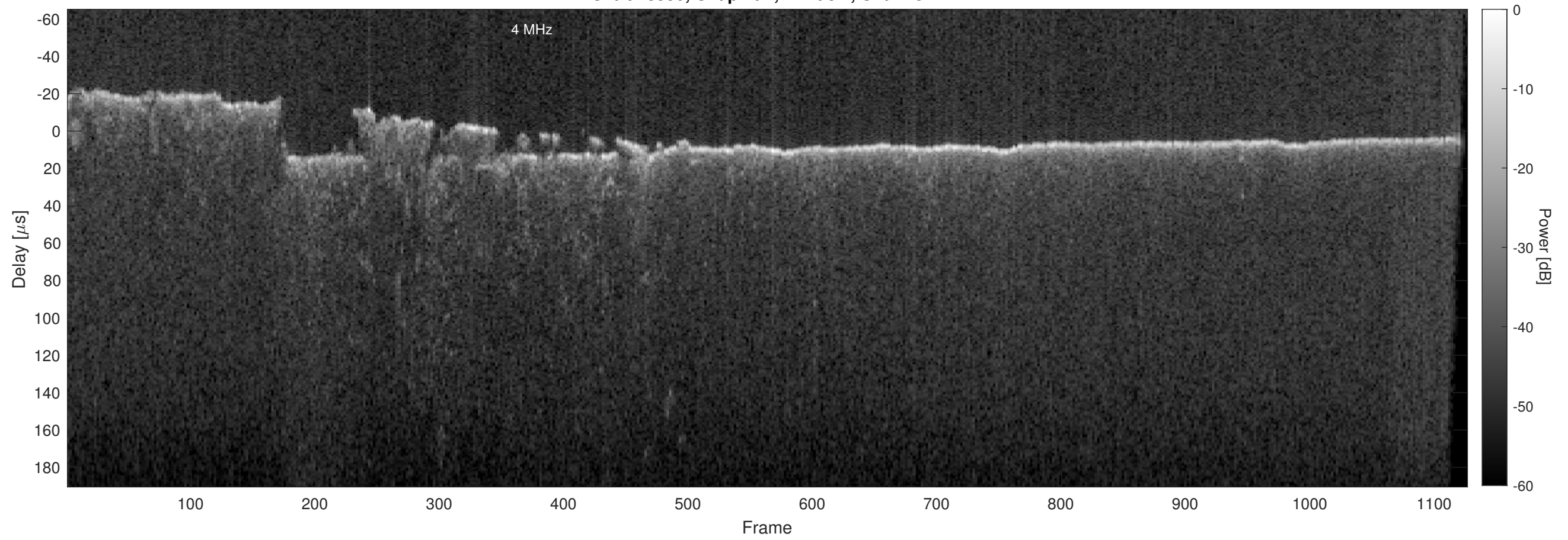
Orbit 18550, Chapman, Window, Channel 2
