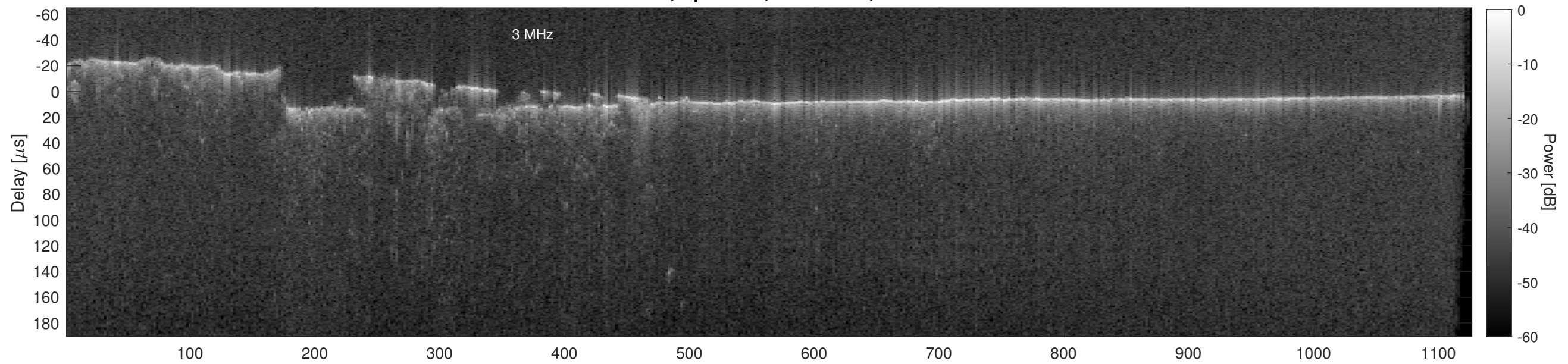
Orbit 18550, Cluttergram
