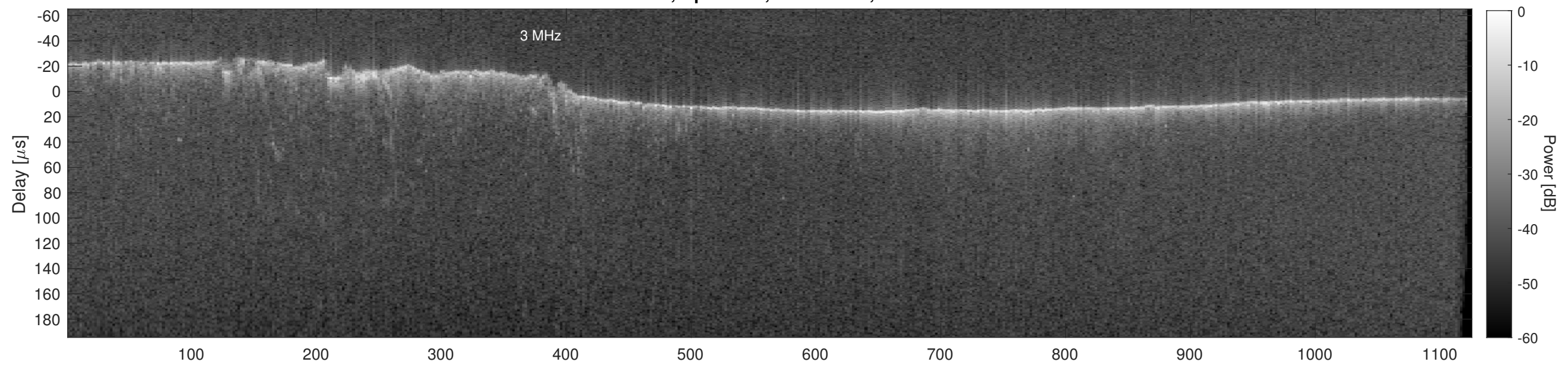
Orbit 18552, Cluttergram
