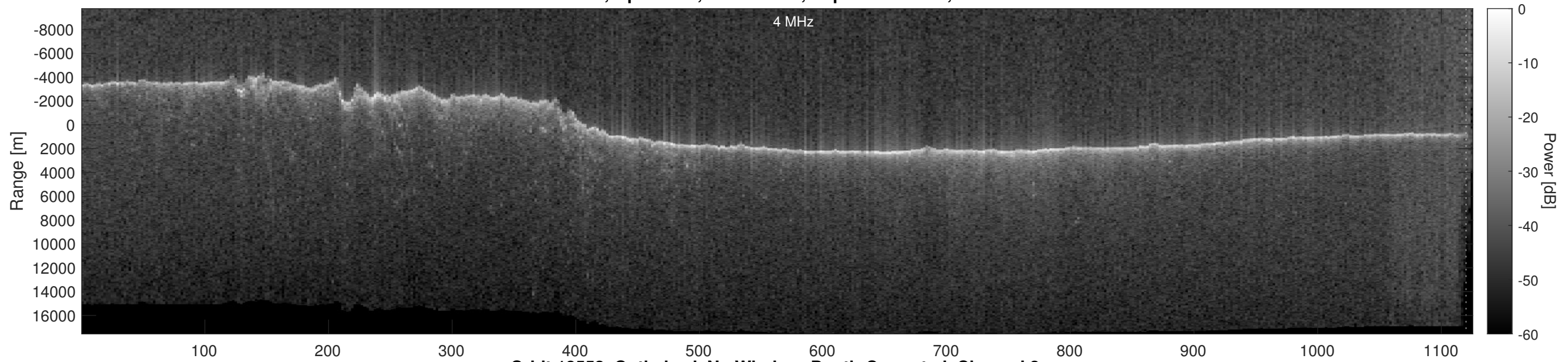
Orbit 18552, Optimized, No Window, Depth-Corrected, Channel 2
