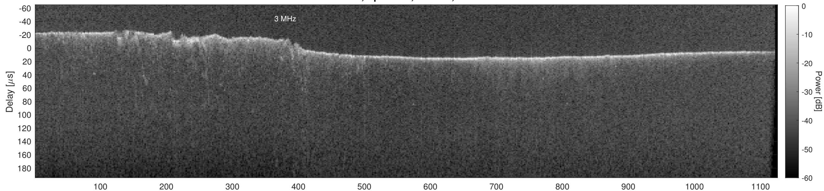
Orbit 18552, Cluttergram
