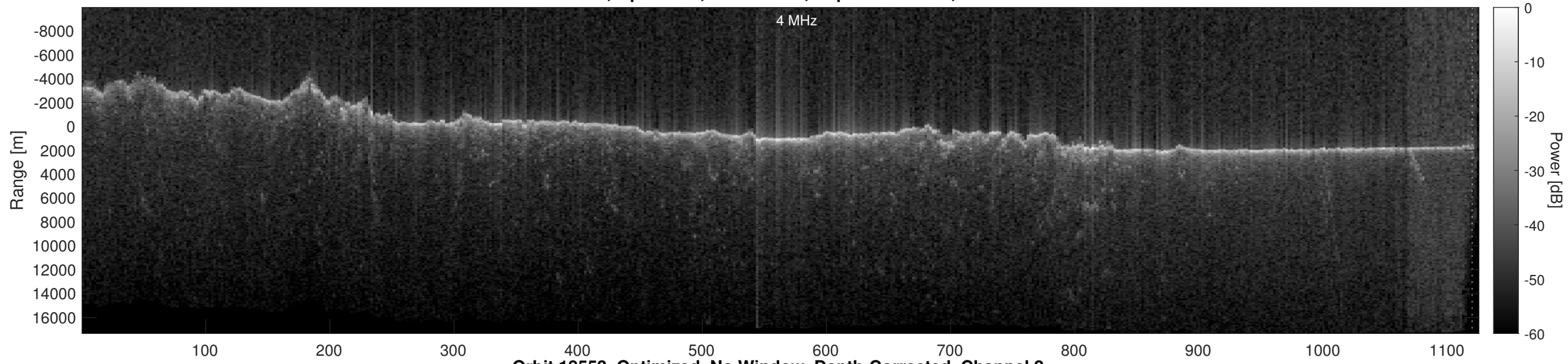
Orbit 18553, Optimized, No Window, Depth-Corrected, Channel 2
