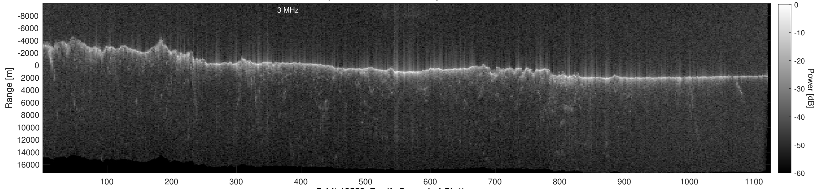
Orbit 18553, Depth-Corrected Cluttergram
