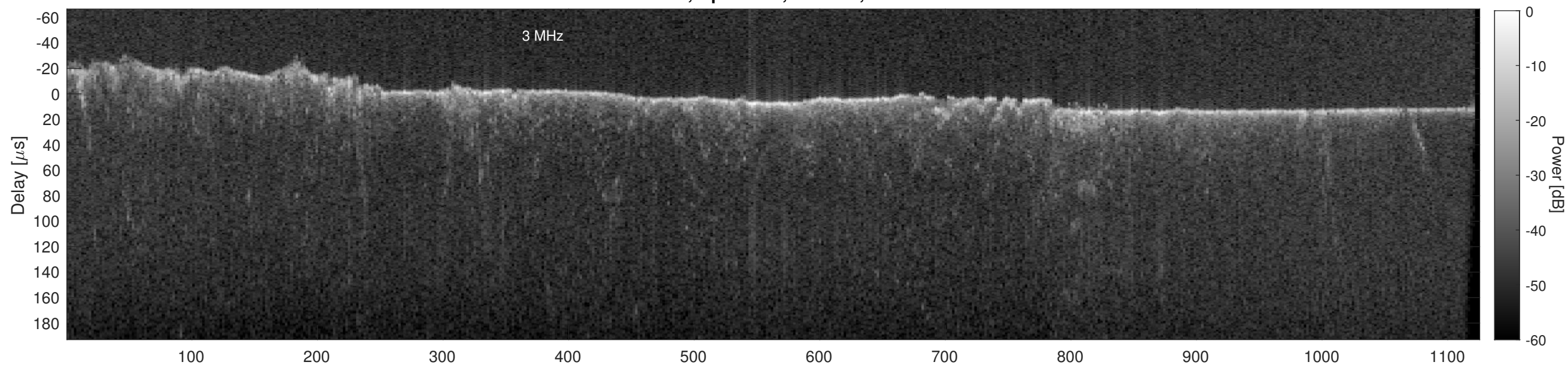
Orbit 18553, Cluttergram
