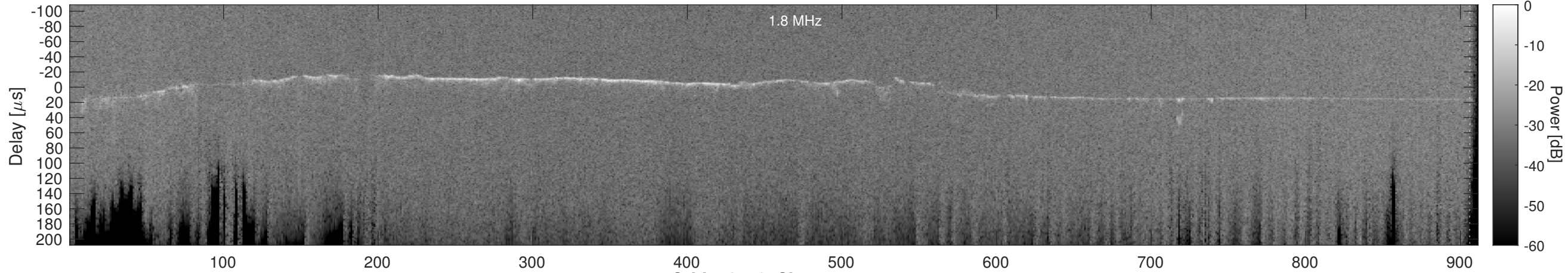
Orbit 18556, Cluttergram
