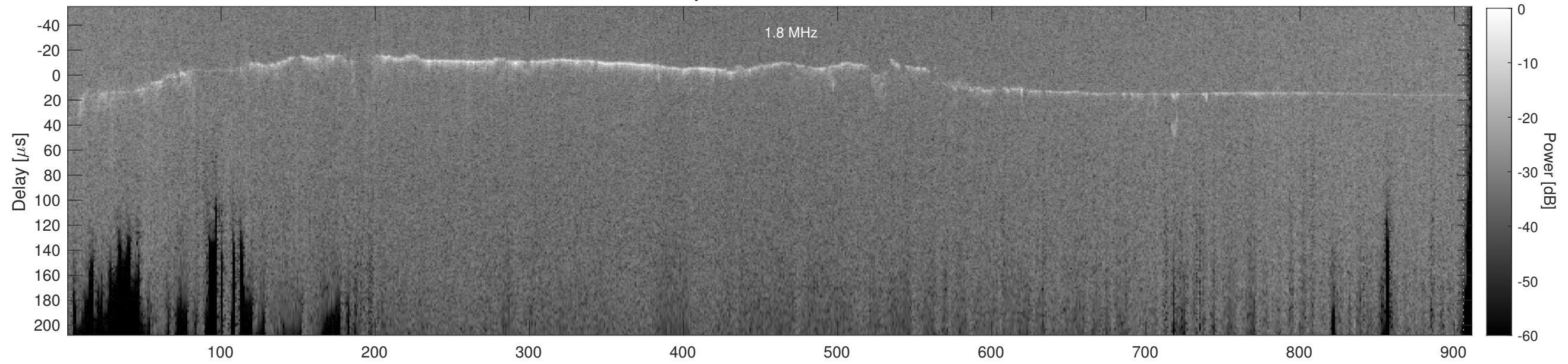
Orbit 18556, Cluttergram
